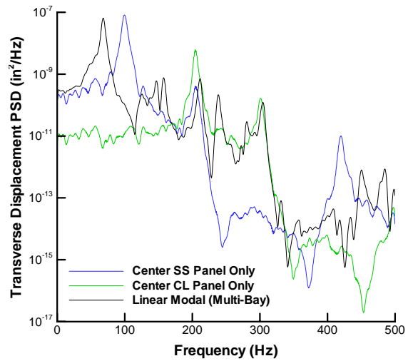
Figure 11: Comparison of multi-bay panel and center bay analyses at 106 dB OASPL.
